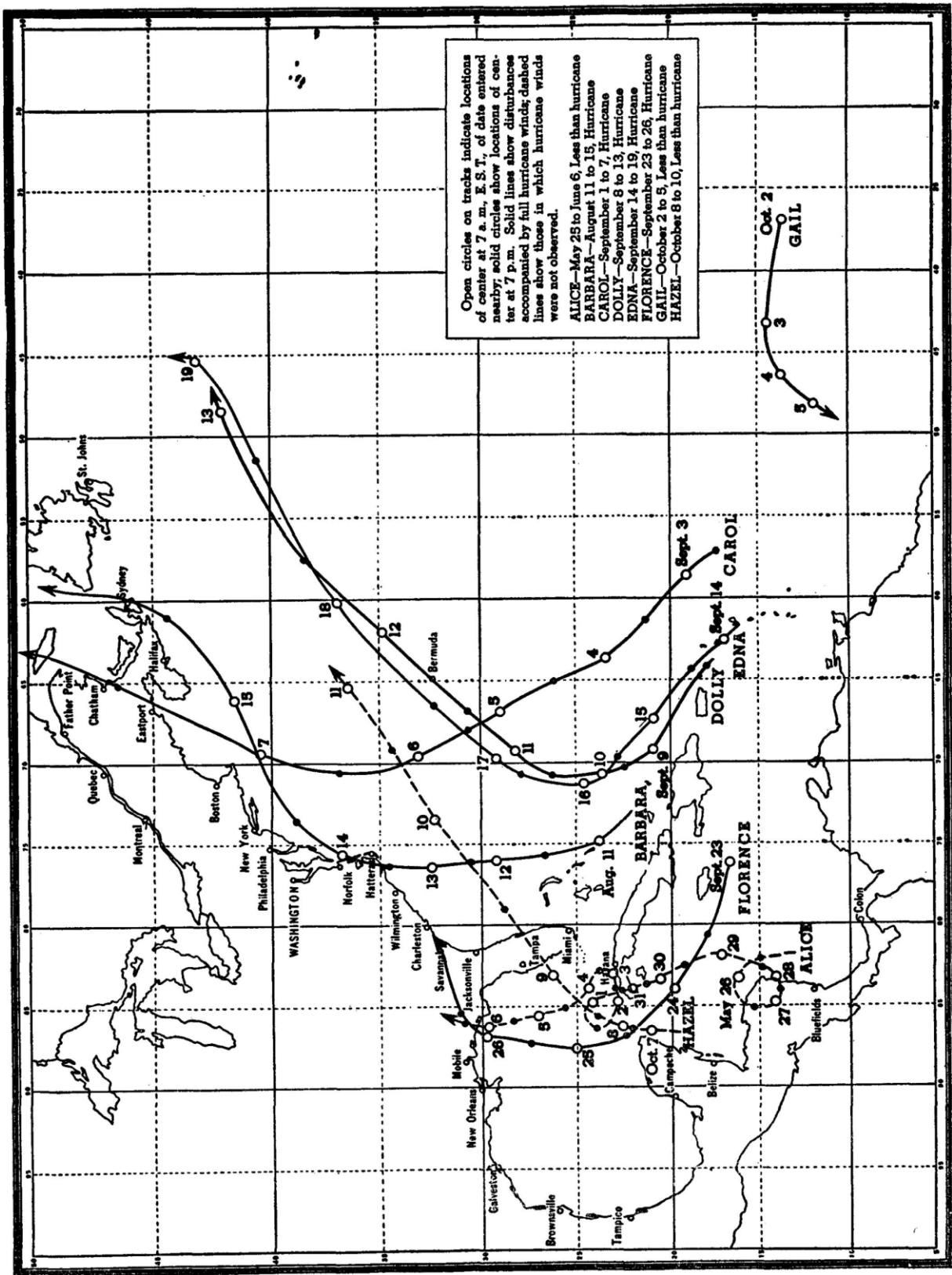
FIGURE 1.—Tracks of hurricanes which occurred during 1963.
