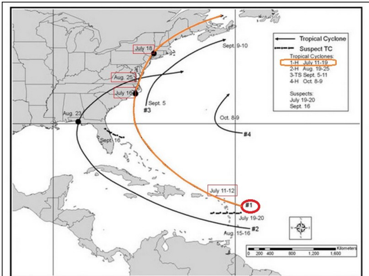
Fig. 1 Track map of the 1850 hurricane season with estimated storm strength and potential suspect storms noted. Solid (dotted) lines indicate confirmed (suspect) tropical cyclones
